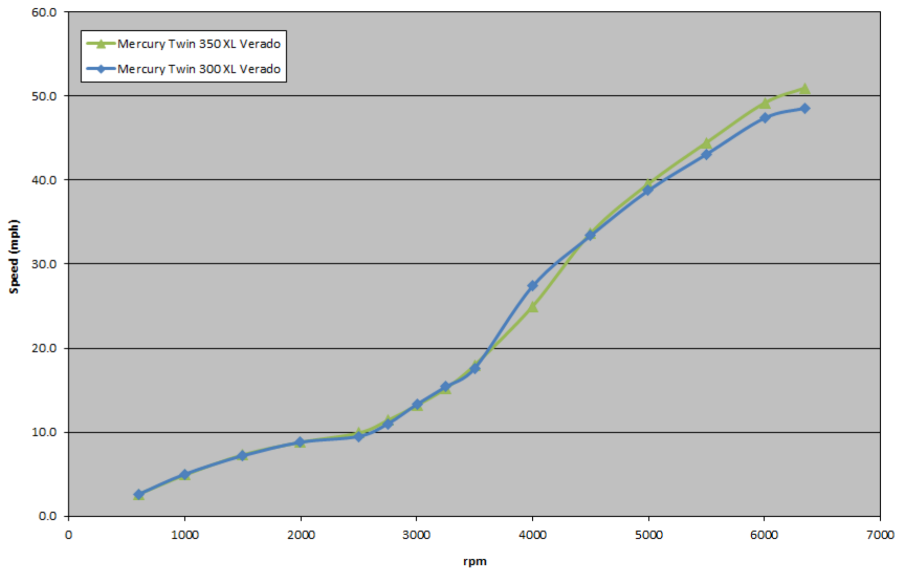
320 Vantage Engine Comparison Graph
