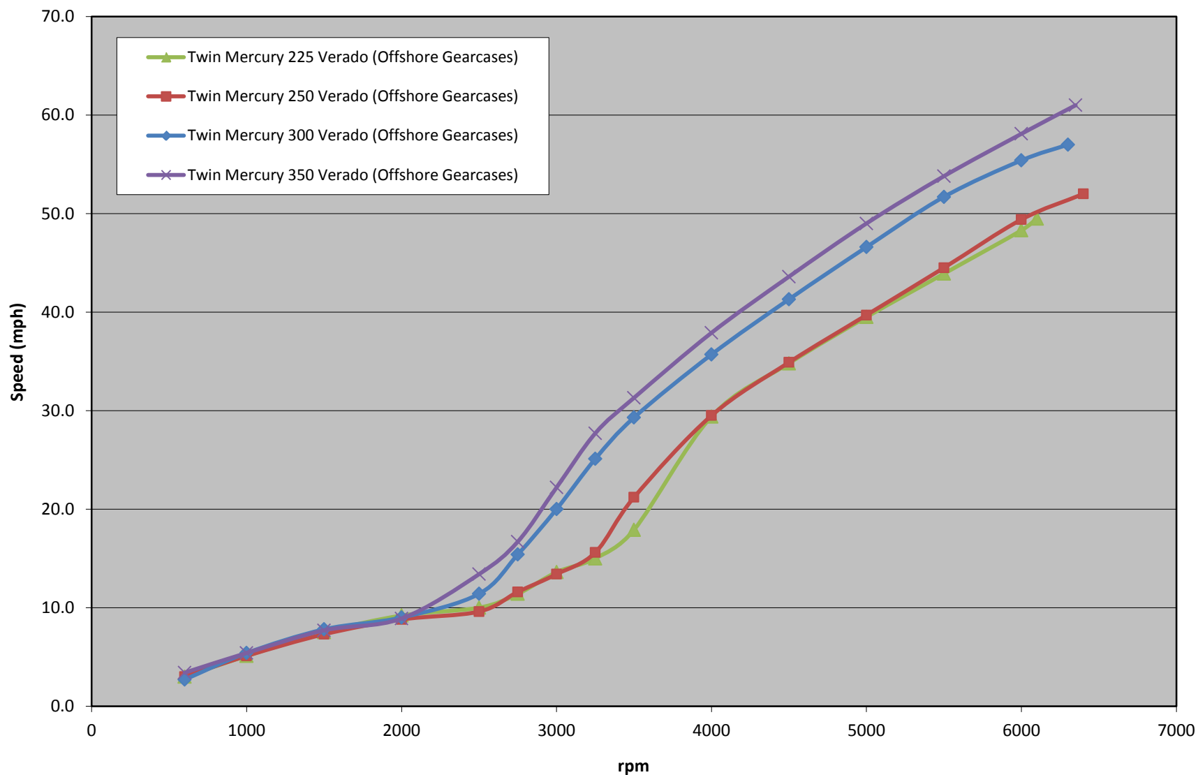
280 Outrage 2016 Engine Comparison Graph
