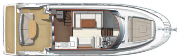
Main deck
